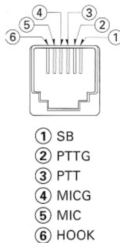
MIC connector (Front view)
