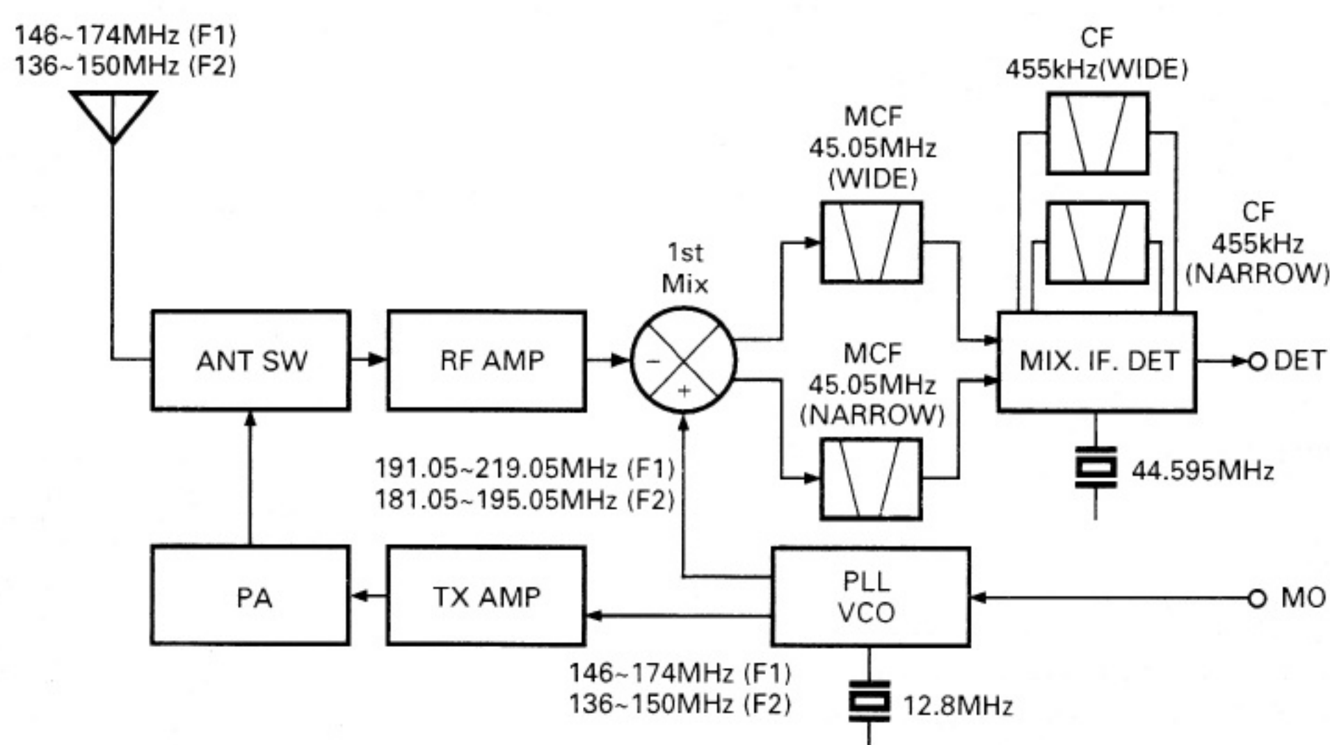
Fig. 1 Frequency configuration
