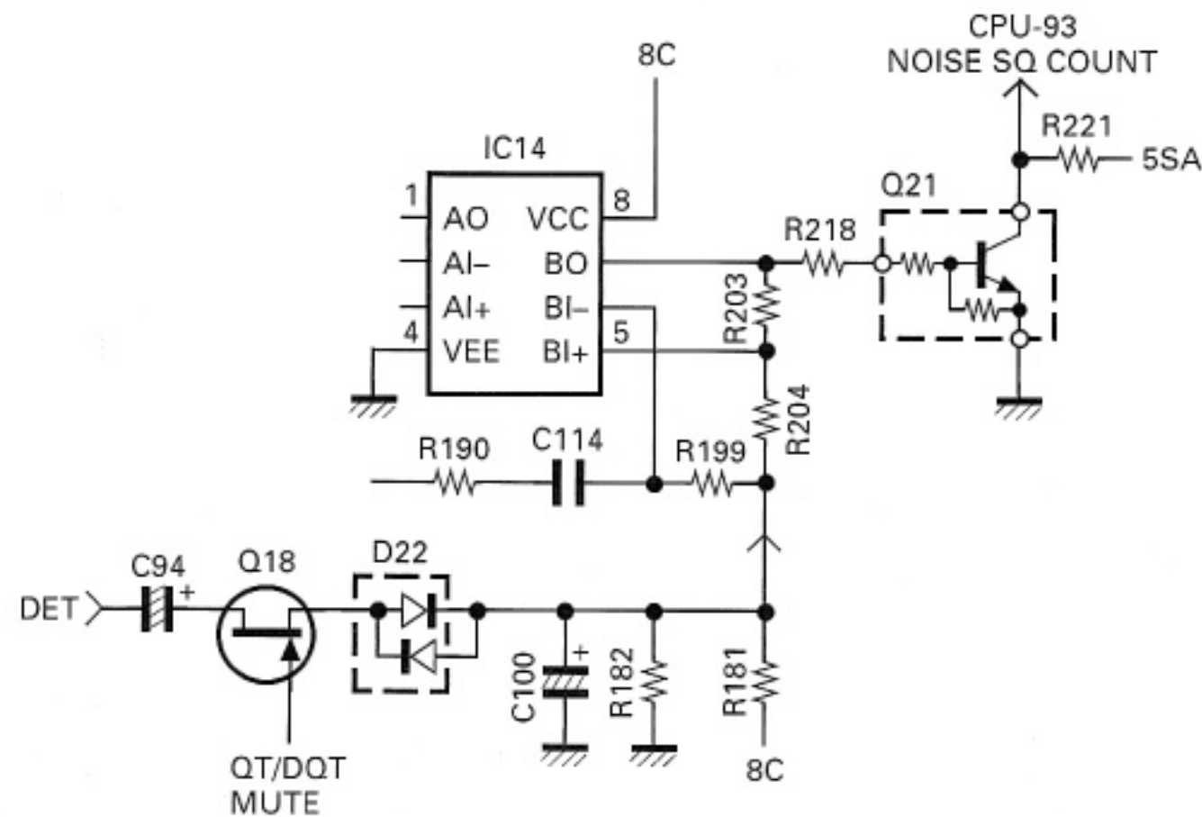
Fig. 4 Squelch circuit
