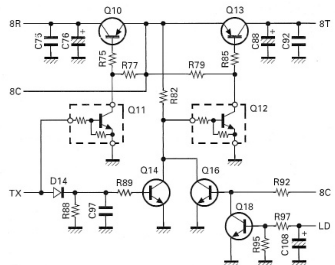
Fig. 10 Unlock circuit
